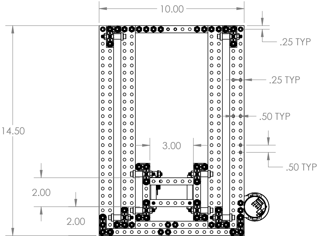
FULLY RETRACTED
