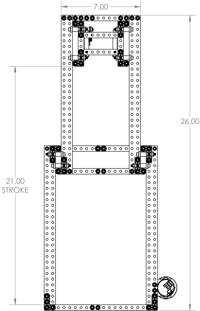
FULLY EXTENDED
