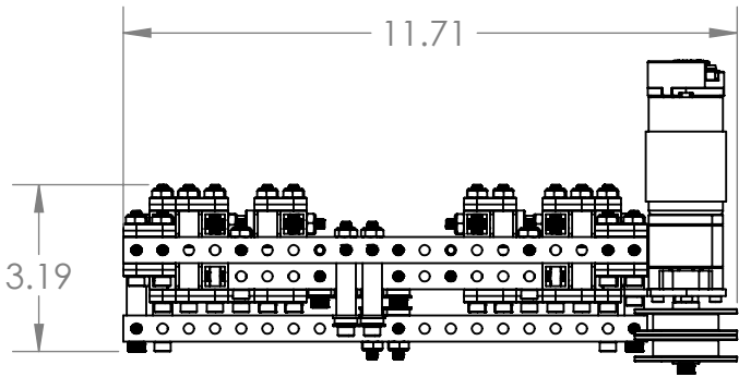
FULLY RETRACTED
